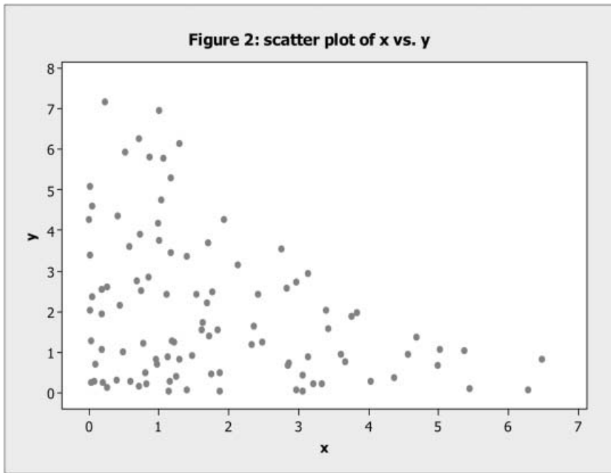
Figure 2 Scatter plot of data \{(x_t, y_t), t = 1, 2, \dots, T\}
