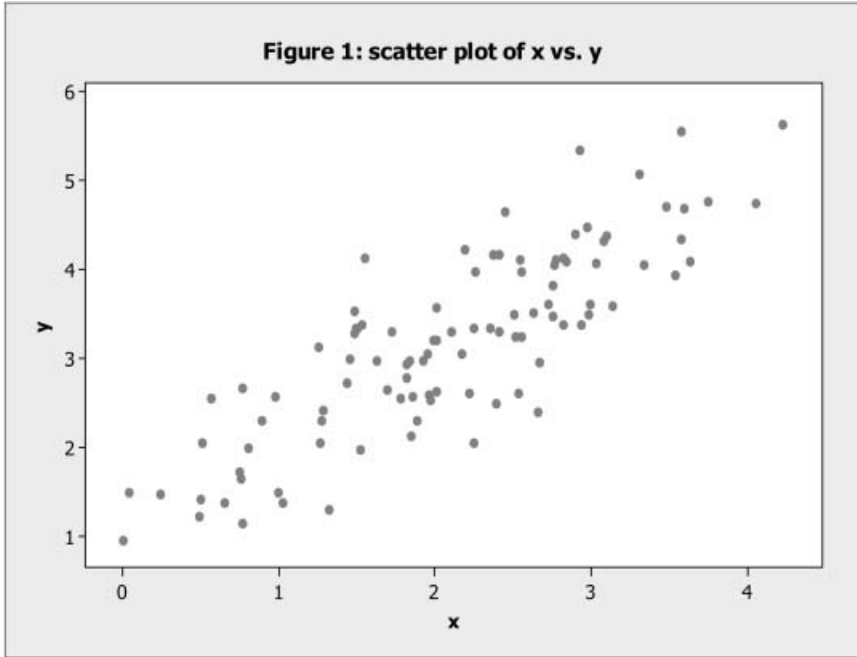
Figure 1 Scatter plot of data \{(x_t, y_t), t = 1, 2, \dots, T\}
