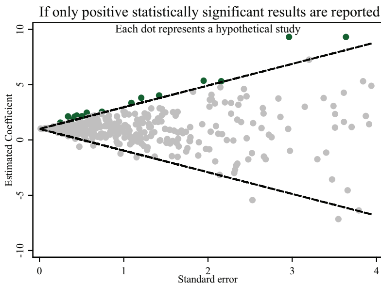
FIGURE 5-3 Funnel charts showing the estimated coefficient and standard error (a) if all hypothetical study experiments are reported and (b) if only statistically significant results are reported.
