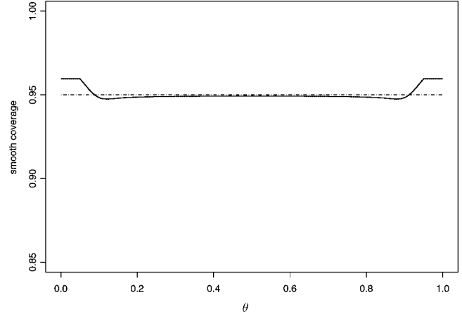
FIG. 2. Local average coverage of the C^{J*} intervals, as a function of \theta when n = 50 and \varepsilon = 0.05 .
